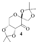
Figure 2. Fructose-derived ketone.
